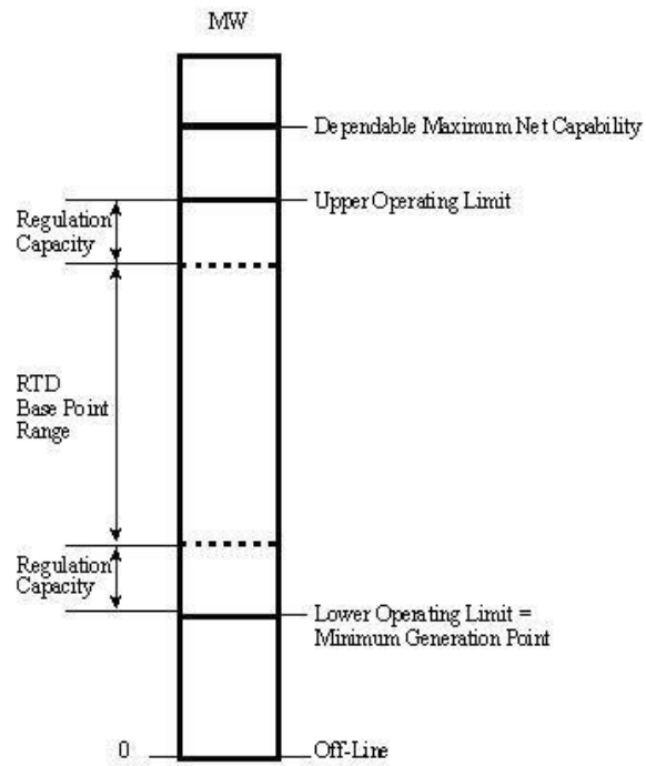
Figure 5: Generating Unit Operating Characteristics
