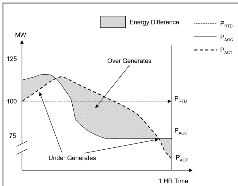
Figure 10: Error in Performance (30-Second Bandwidth not Included)
