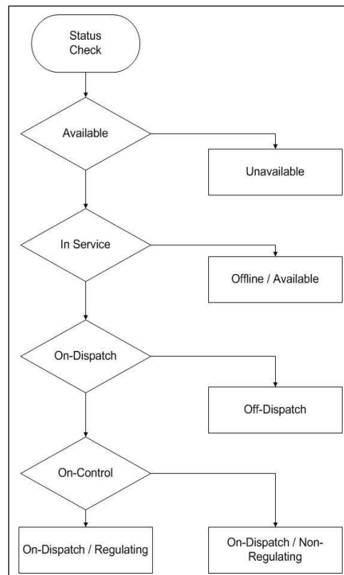
Figure 8: Generating Unit Operating States
