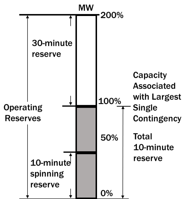
Figure 11: Minimum Operating Reserve Requirements
